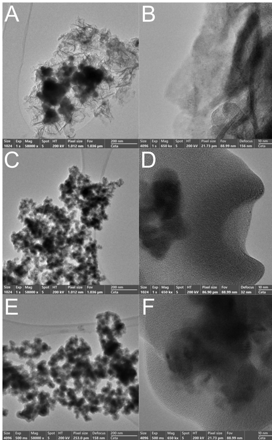
Fig. 1 HR-TEM images at low (left column) and high (right column) magnification (58 Kx and 650 Kx) of NiGrif NG1-2-3 samples with increasing load of graphene oxide: (A) and (B) 0.2% GO, (C) and (D) 1% GO, (E) and (F) 5% GO. Scale bar of 200 nm for the low magnification (left column) and 10 nm for the high magnification (right column).
