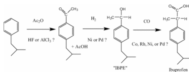
Scheme 2. General Synthetic Strategy for “Profen” Drugs Developed by Murphy at Celanese in 1984. IBPE Stands for 1-(4-Isobutylphenyl)ethanol. [Reproduced from Ref 50, Creative Commons CC BY license]
